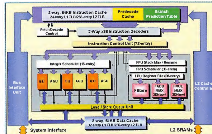
This flow-chart actually means something. It's of the instruction set for AMD's 'Athlon' K7 chip.
